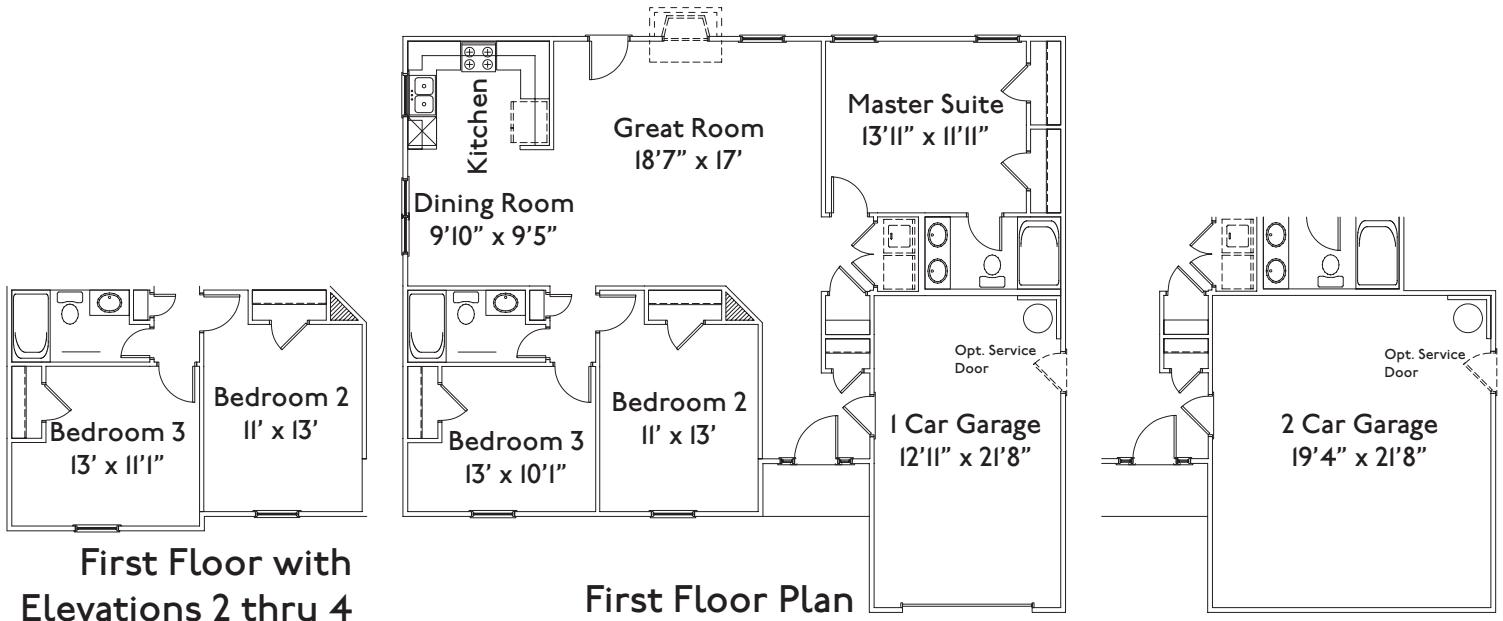
First Floor with Opt. 2 Car Garage
