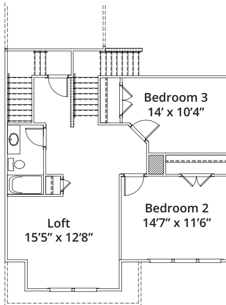
Second Floor Plan w/ Opt. Bonus Room
