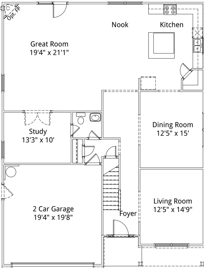
Main Level
