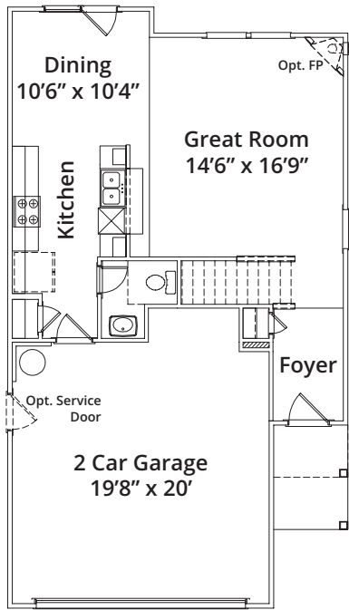
Main Level
